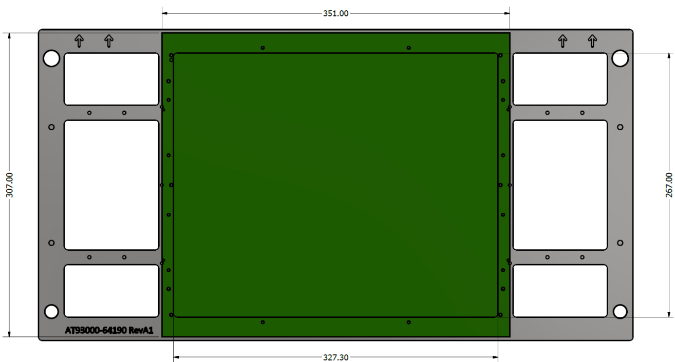
Figure 5. Stiffener Application Space Area Dimensions
